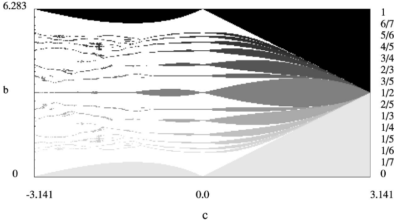
FIG. 1. Distribution of rotation numbers of the circle map (1). Several regions where the rotation numbers are rational ( \rho = p/q ) are presented. From the bottom to the top the different gray level regions are ordered as shown on the right side. Between these regions there exist (but not presented) relatively small regions with other rational rotation numbers.
